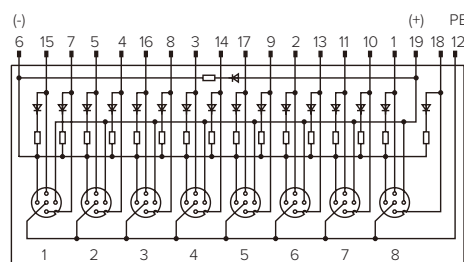
Wiring Diagram
